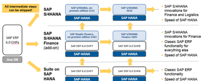
SAP S/4 HANA Upgradepfade
